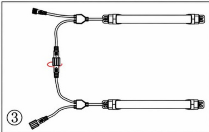
3. Tighten the nut of the connector.
