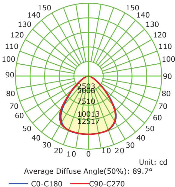
Luminous Intensity Distribution Curve 160170 180 170160
